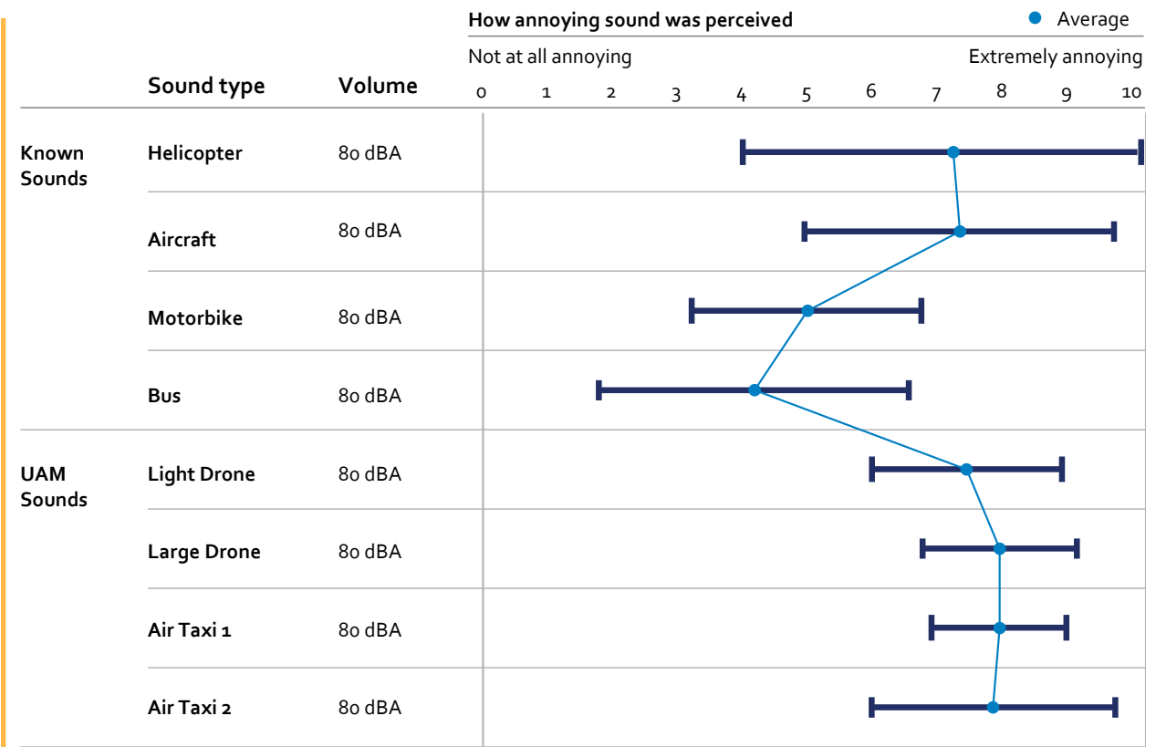
Figure 48: Result comparison between familiar sound and Urban Air Mobility vehicle sounds at same maximum noise level
